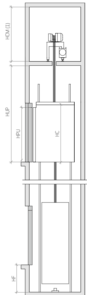
VERTICAL SECTION
